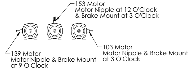
Explosion Proof Motor Identification Viewed from Motor Shaft End
